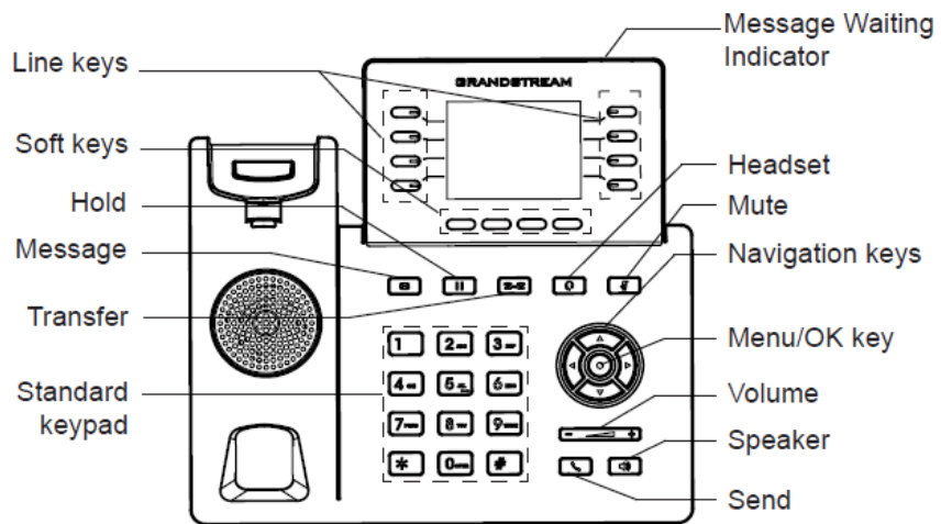
Figure 11: GRP2624 Keyboard
