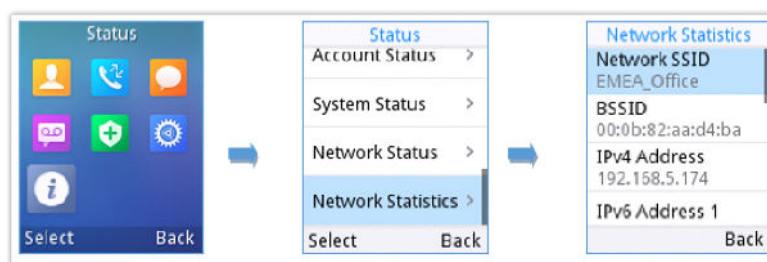
Figure 23: Network Statistics
