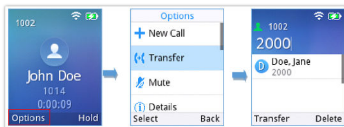
Figure 39: Blind Transfer
