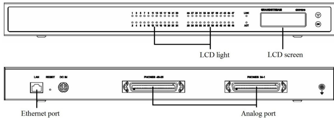
Figure 1: Diagram of GXW4216/24/32/48 Panel
